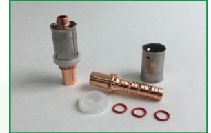
MALE FITTING
